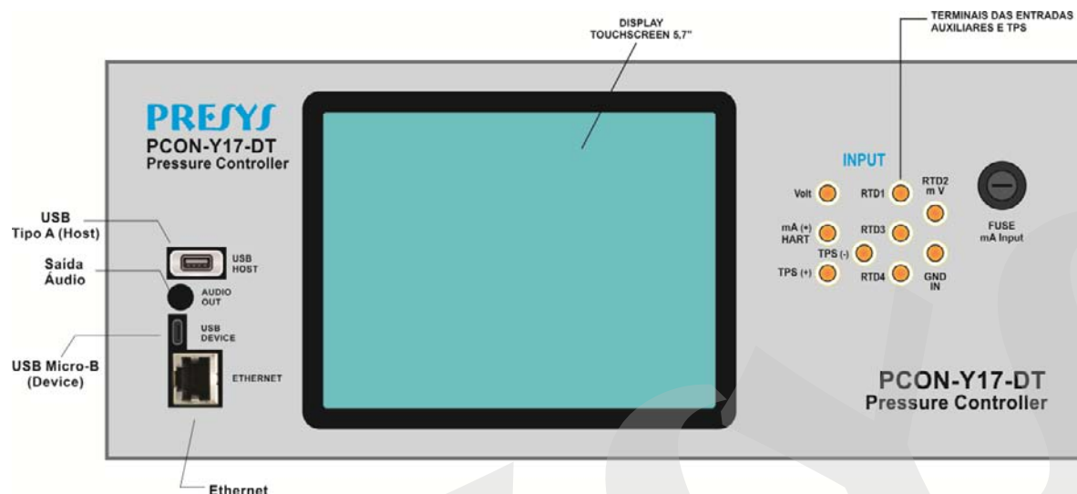
Fig. 01 - Painel Frontal PCON-Y17-DT
