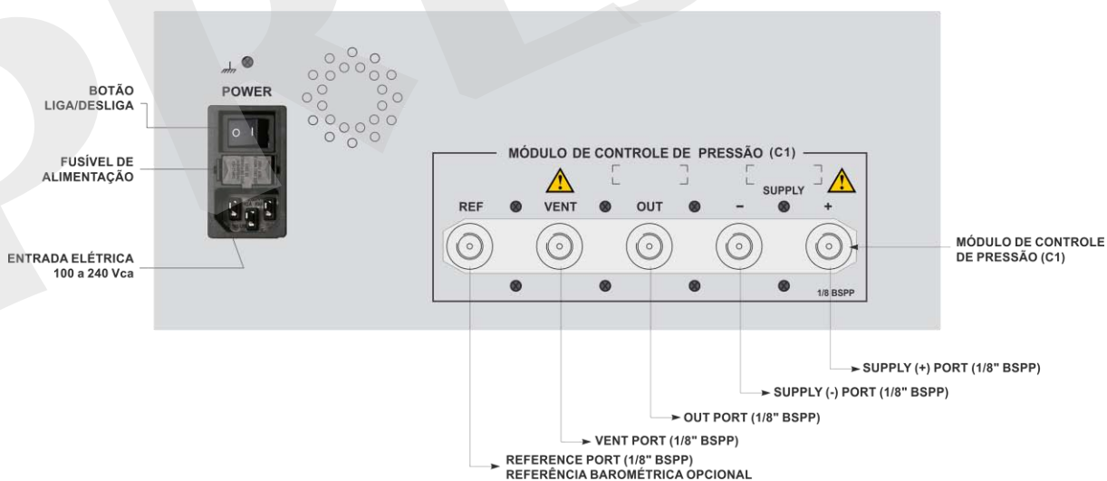
Fig. 02 - Painel Traseiro PCON-Y17-DT
