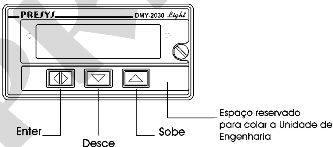
Fig. 1 - Painel frontal do indicador DMY-2030 Light -Energy
