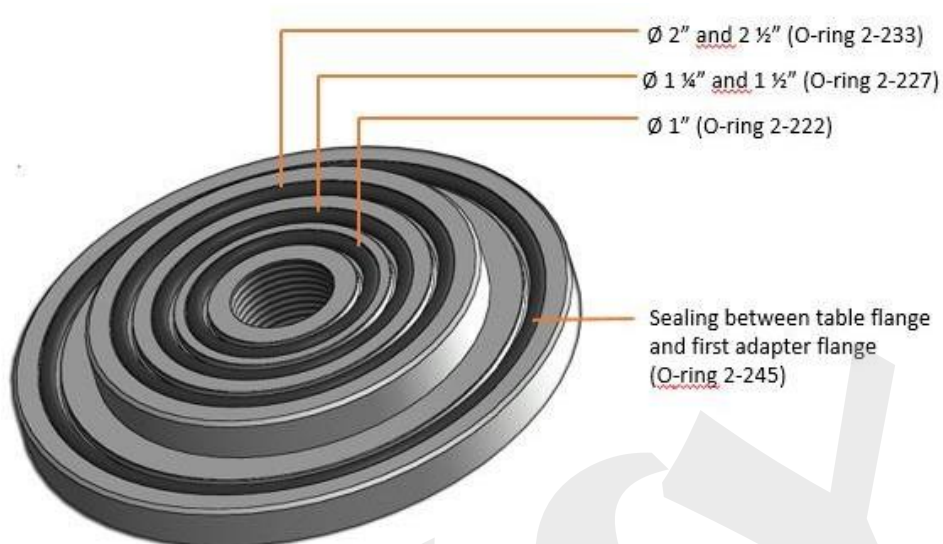
Fig. 25 - Flange Central
